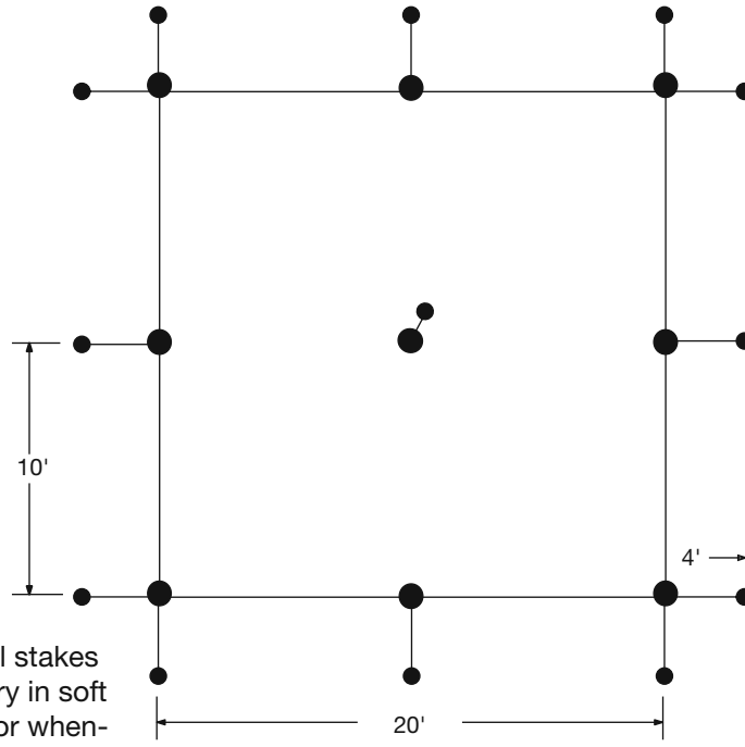
PLAN W/STAKES
