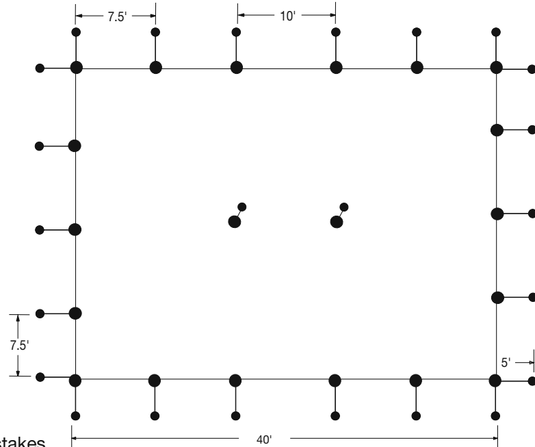
PLAN W/STAKES
